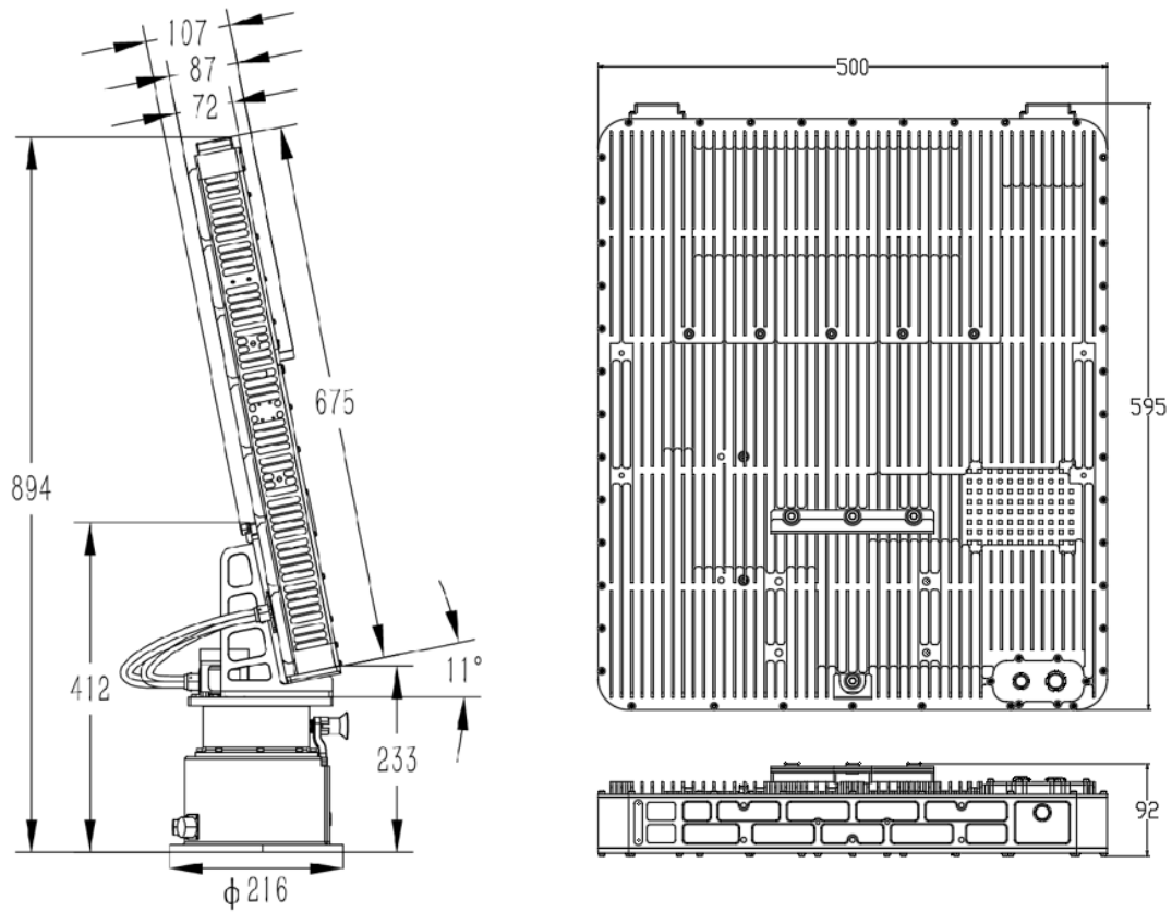
CR-FX10 structural and installation dimensions (unit: mm)
