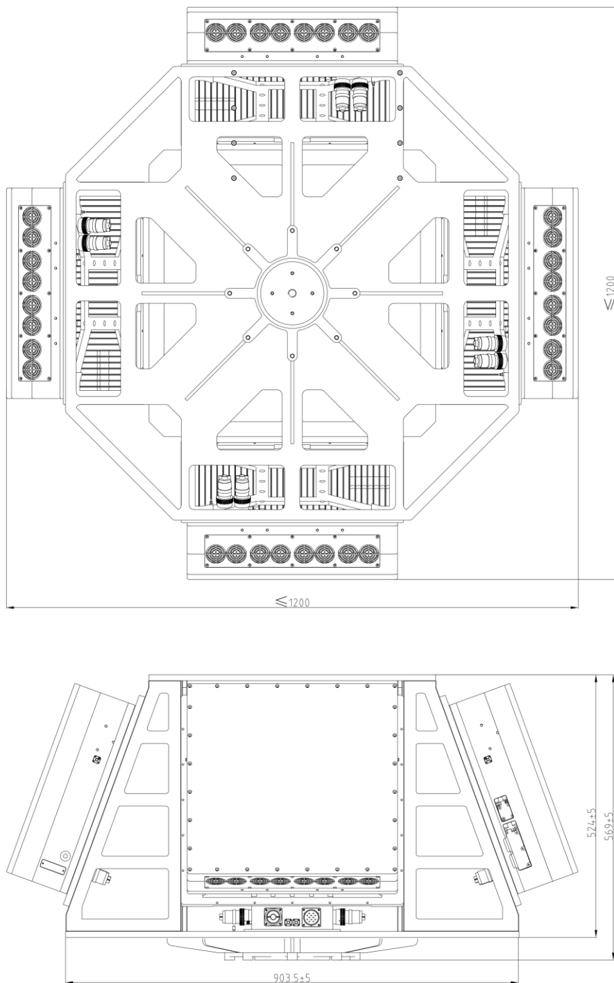
CR-PK14C structural and installation dimensions (unit: mm)
