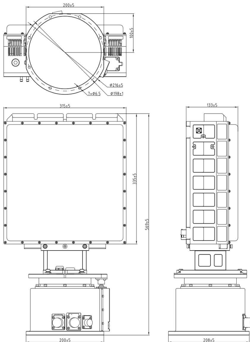
CR-PX08B structural and installation dimensions (unit: mm)
