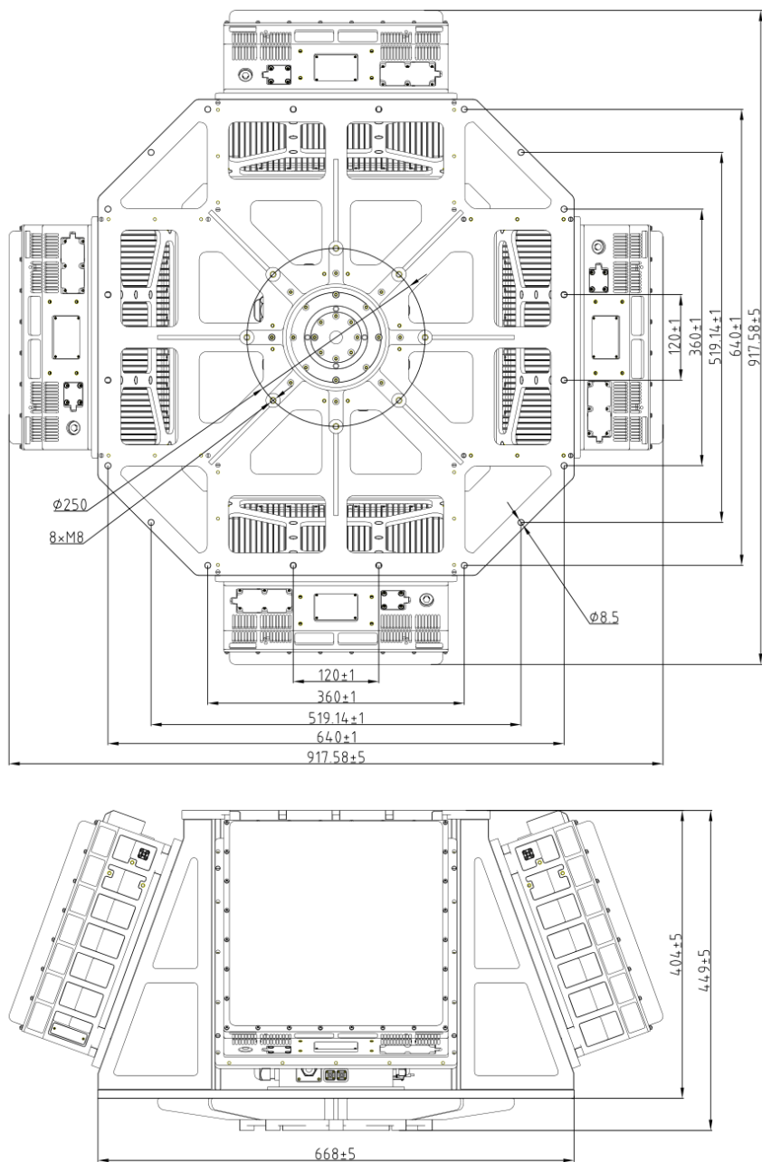
CR-PX08C structural and installation dimensions (unit: mm)
