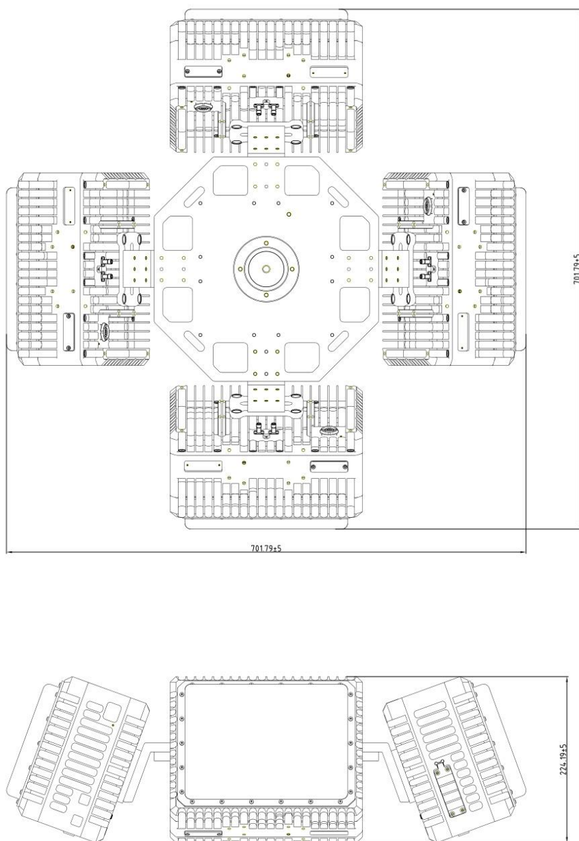
CR-PX10C structural and installation dimensions (unit: mm)
