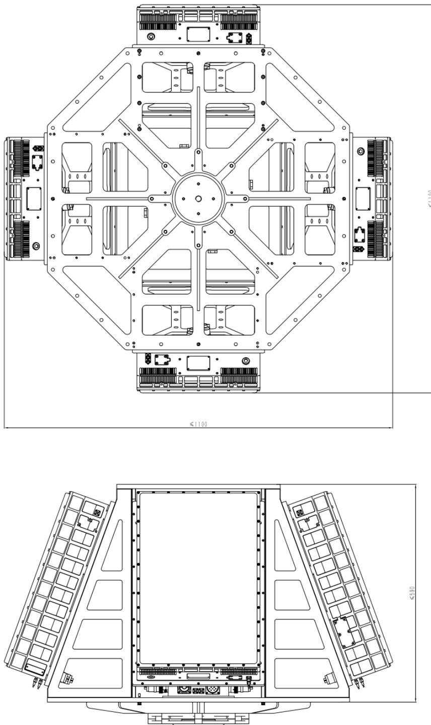
CR-PX11C structural and installation dimensions (unit: mm)
